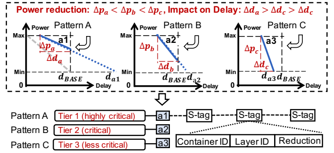
Figure 9: The mechanism for ranking microservices.
